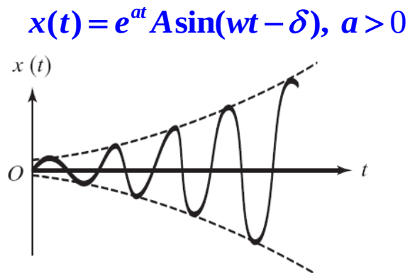
Unstable system (with flutter instability) (擺動)
