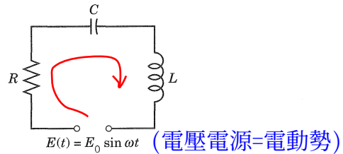
Fig. 61. RLC-circuit
