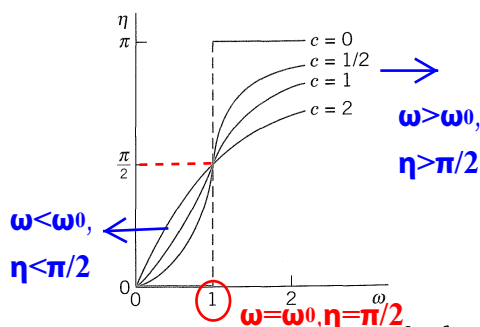
Fig. 58. Phase lag \eta as a function of \omega for m = 1 , k = 1 , thus \omega_0 = 1 , and various values of the damping constant c
