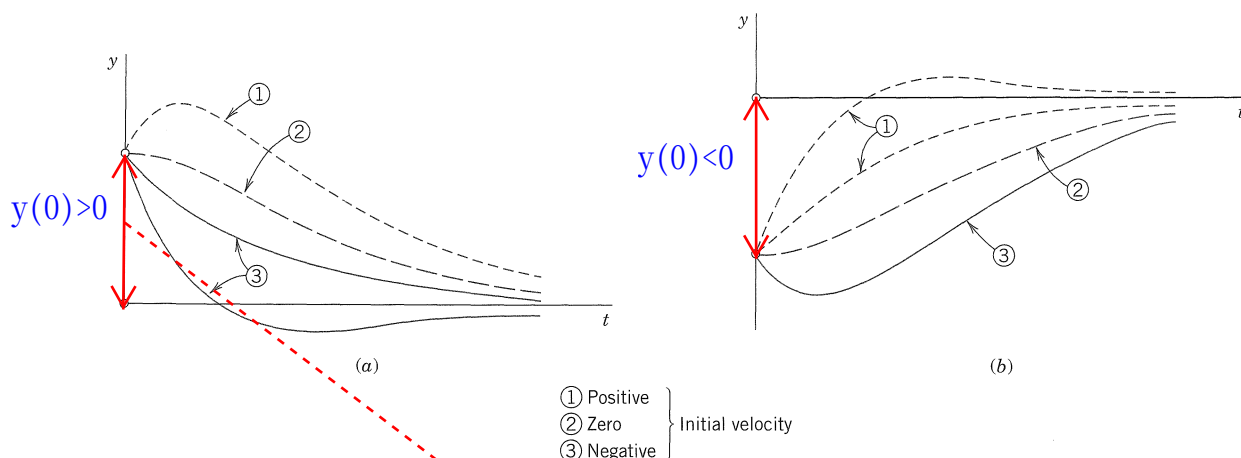
Fig. 37. Typical motions (7) in the overdamped case (a) Positive initial displacement (b) Negative initial displacement
