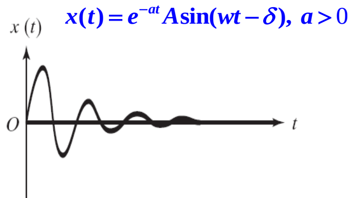
Asymptotically stable system (漸進的)
