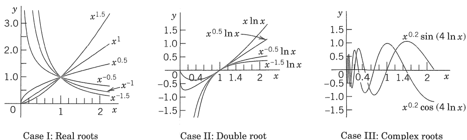
Fig. 48. Euler–Cauchy equations
